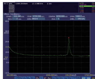
Measurement example of wavelength loss characterization
